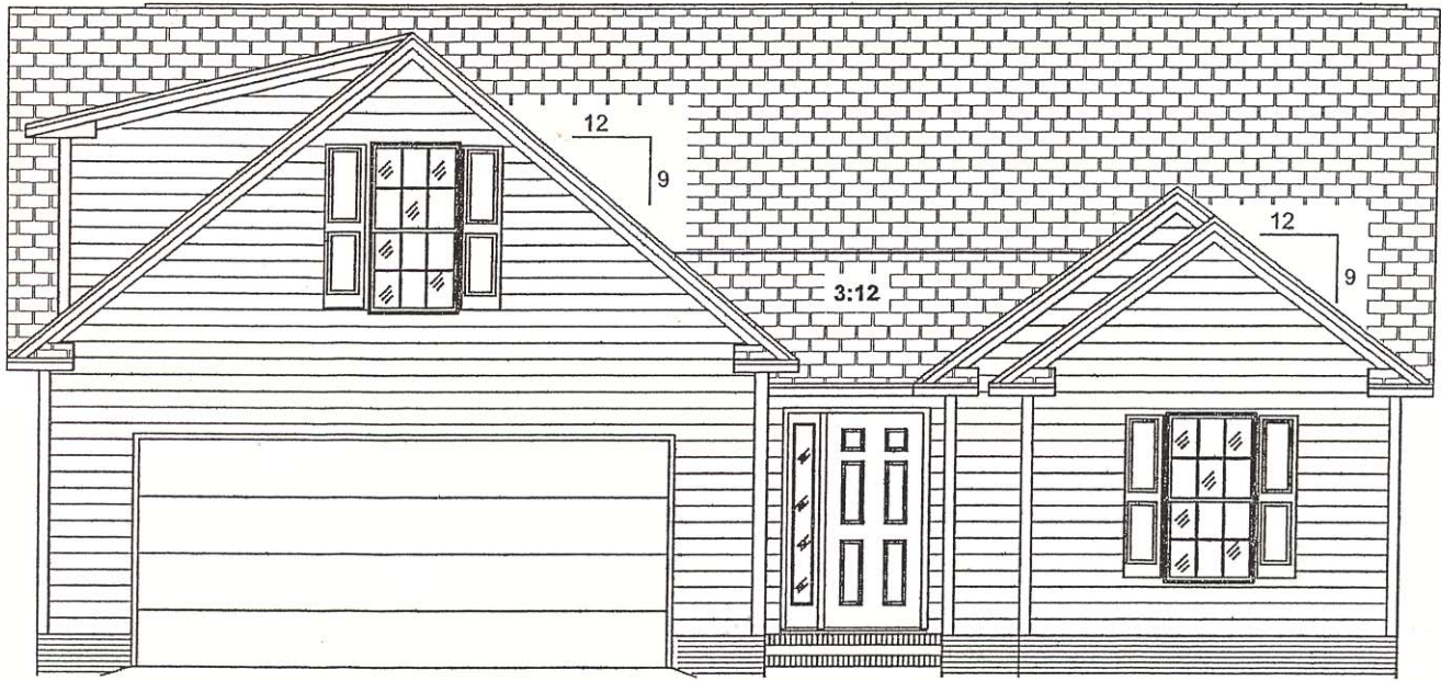
FRONT ELEVATION
